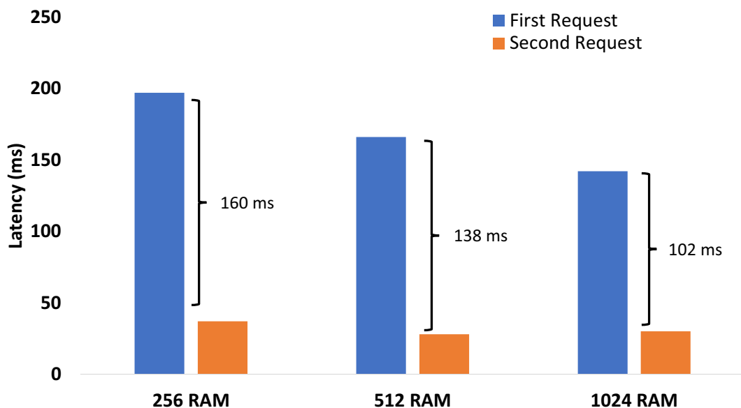
Fig. 11 The impact of different main memory capacity (RAM) on cold start latency
