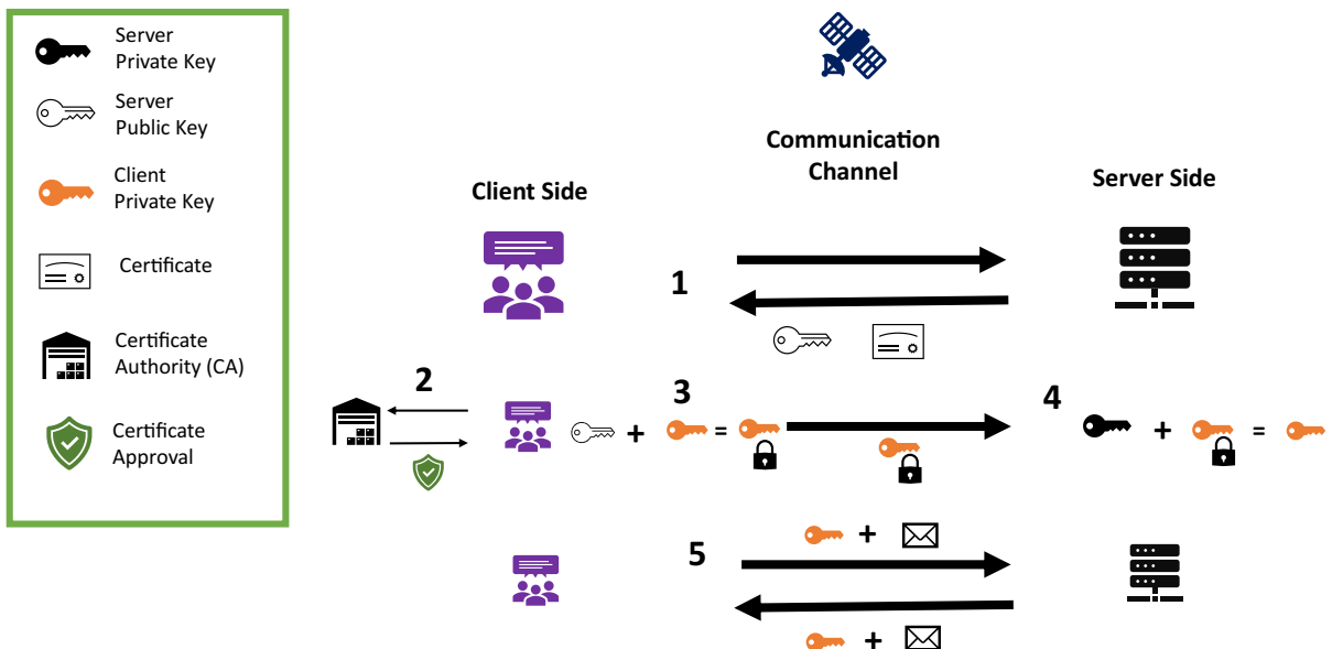
Fig. 3 TLS protocol mechanism
