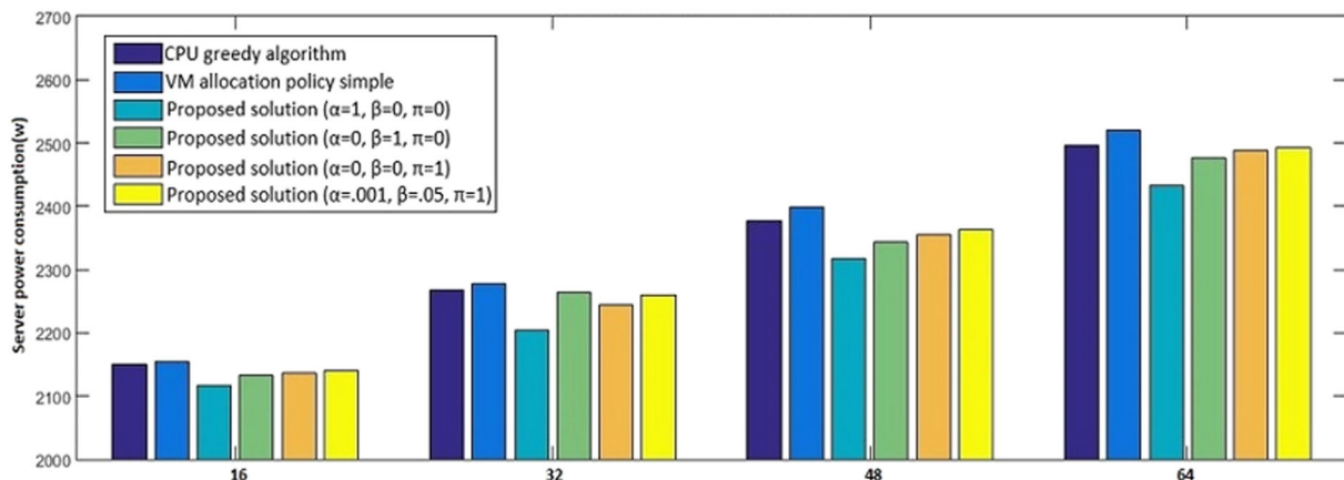
FIGURE 10 Comparison of the physical machines power consumption (watt) in three-tier topology
