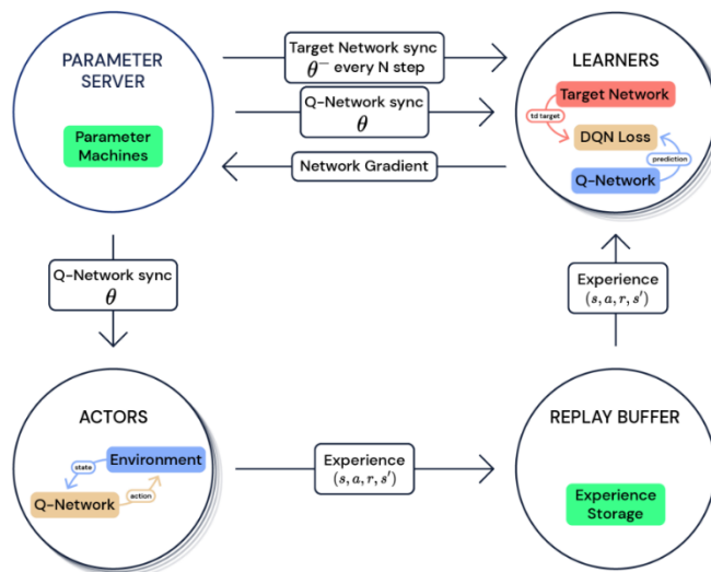
GORILA Architecture
